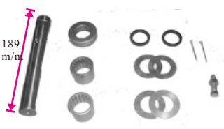
TOYOTA 8FD25
